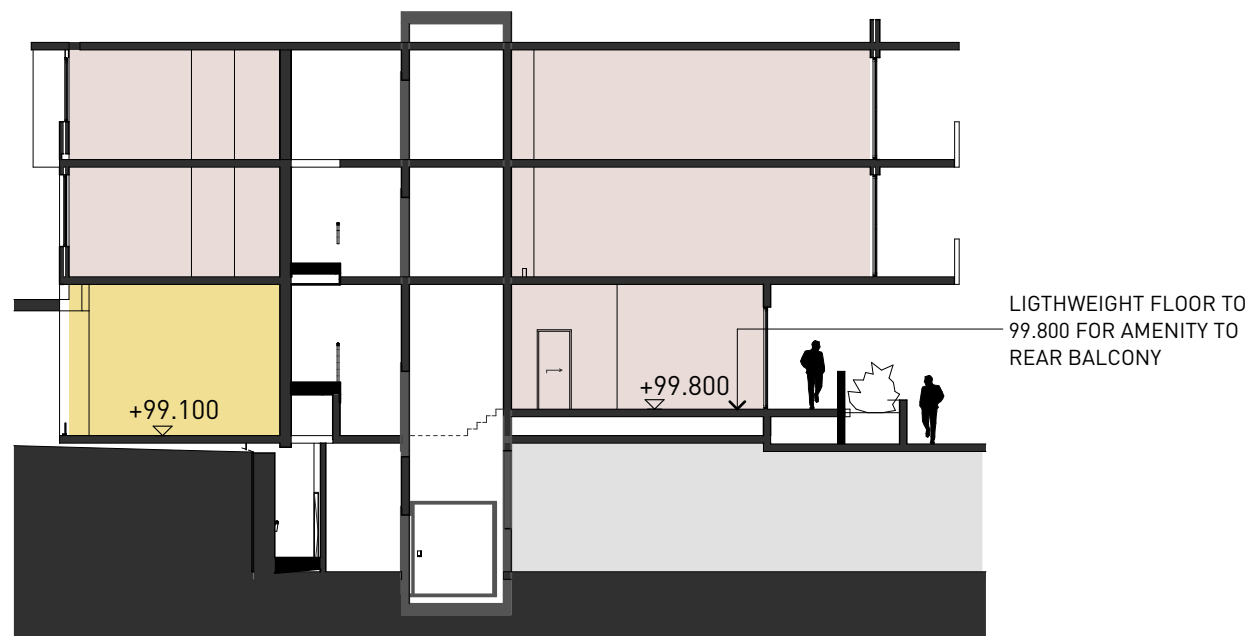
3 SECTION A 1:200
