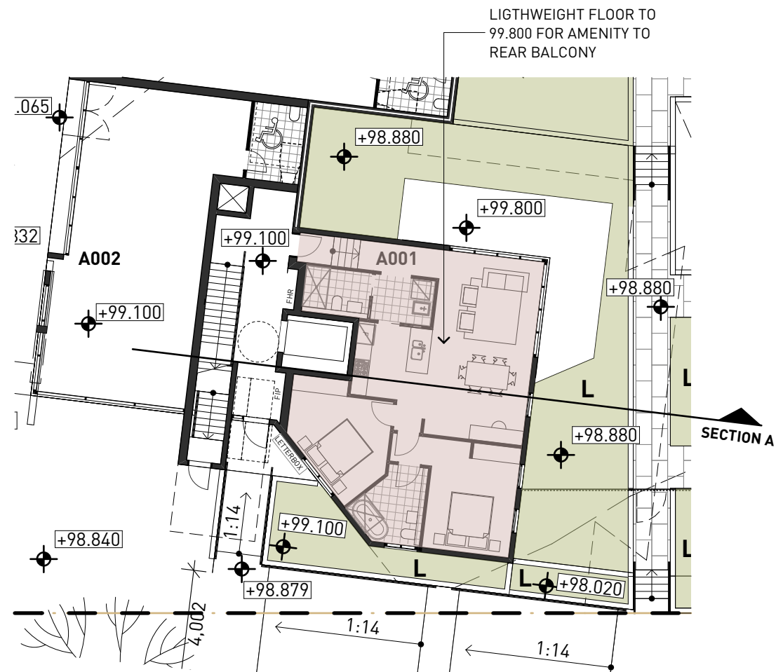
1 PLAN LEVEL 0 - RESIDENTIAL USE 1:200
